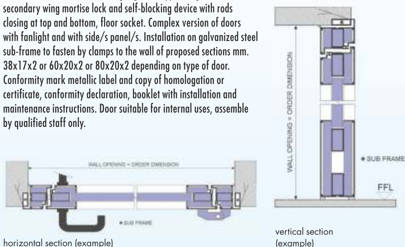
horizontal section (example)
