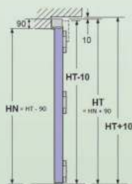
Vertical section single and double leaf with tubular frame
