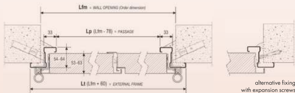
horizontal section
