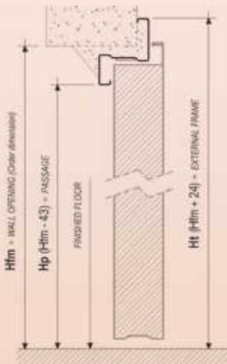
vertical section of handed doors
