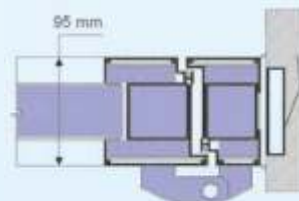
95 mm. aluminium covered profile
