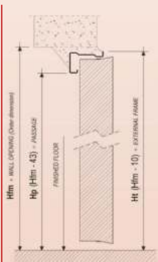
vertical section of reversible doors
