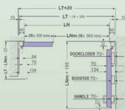
Horizontal section double leaf with tubular frame
