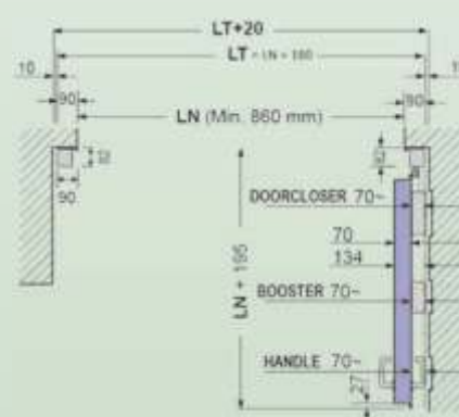
Horizontal section single leaf with tubular frame
